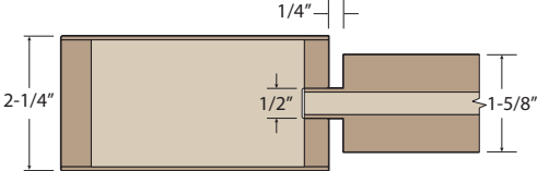
2-1/4" Profile with Square Stick (SS) sticking and Senior Flat (H) panel
