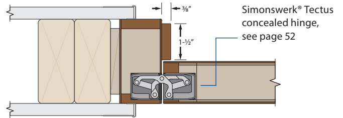
Jamb detail of drywall return jamb with concealed hinge Compatible with standard barrel hinges. Jamb must be installed before applying drywall
