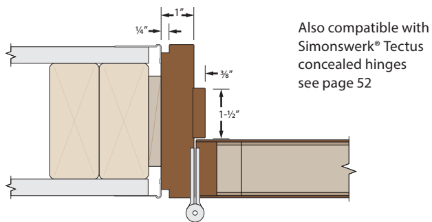
Jamb detail with L-bead trim and barrel hinge Also available in single rabbet configuration.
