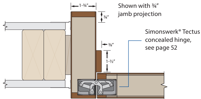
Jamb detail with L-reveal trim and concealed hinge Compatible with standard barrel hinges.
