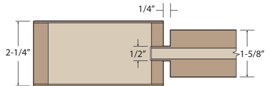
2- \frac{1}{4} " Profile with Square Stick (SS) sticking and Senior Flat (H) panel
