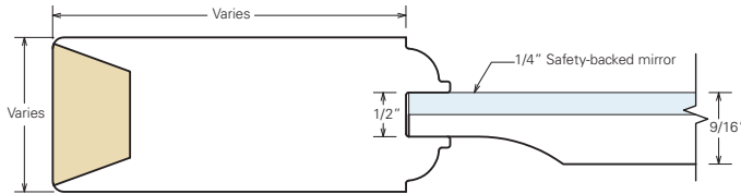
Sample cross section (one-sided mirror door)
